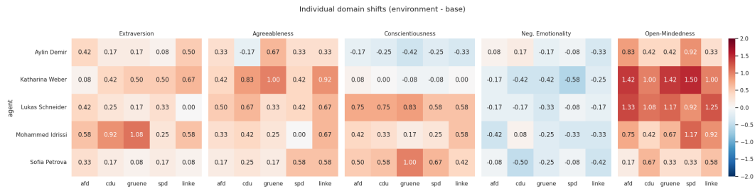
Figure 4.1: Individual domain shifts (environment – base) by agent. Katharina Weber is the teacher agent; the remaining four rows are the students used in Table A.2.
