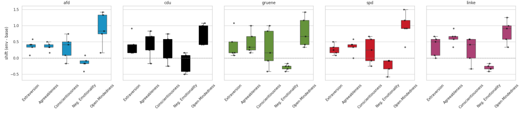
Figure 4.2: Spread of individual student shifts per domain, one panel per environment.
