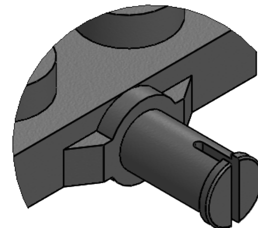
DETAIL C SCALE 6 : 1
