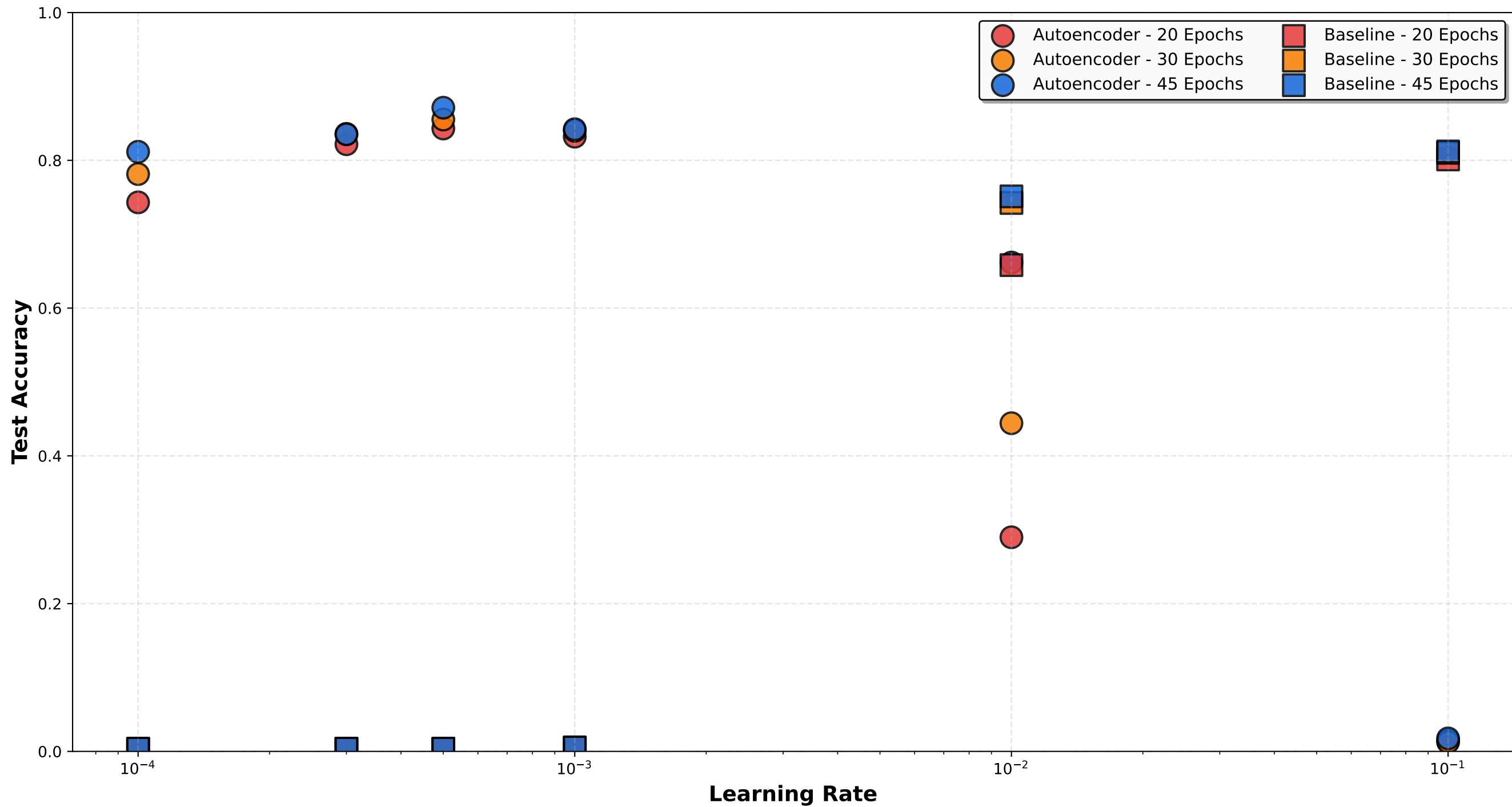
Test Accuracy Comparison: Baseline vs Autoencoder Classifier
