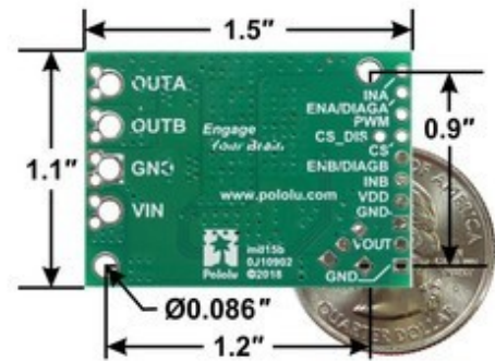
VN15019 motor driver carrier, bottom view with dimensions.
