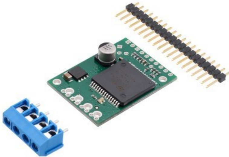
VNH5019 motor driver carrier with included hardware.
