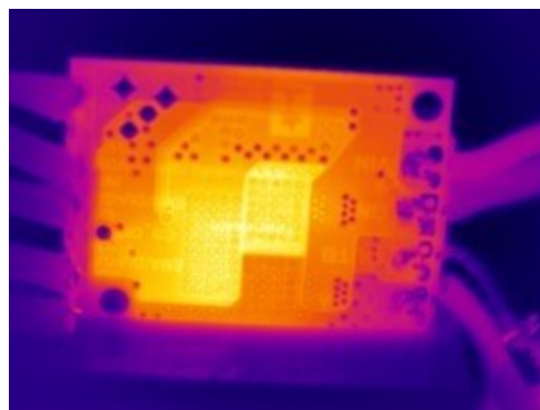
Thermal image of the underside of the VNH5019 motor driver carrier during one of our current tests.
