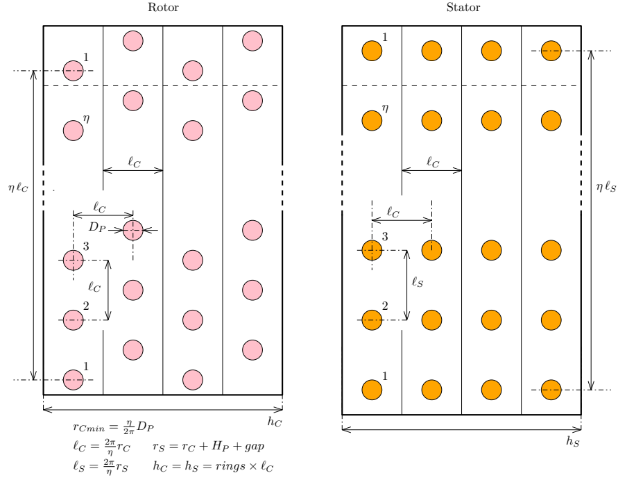
Fig. 4: Flat view of stator and staggered rotor rings. Notice that the ratio height to diameter ( = h_C/2r_C ) of the rotor cylinder turns out to be \frac{rings}{\eta}\pi .
