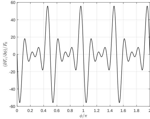
Fig. 9: Normalized \Gamma(\phi) in (6) with \eta = 16 . It results in \text{MAX}\{\Gamma(\phi)\} = 56 .
