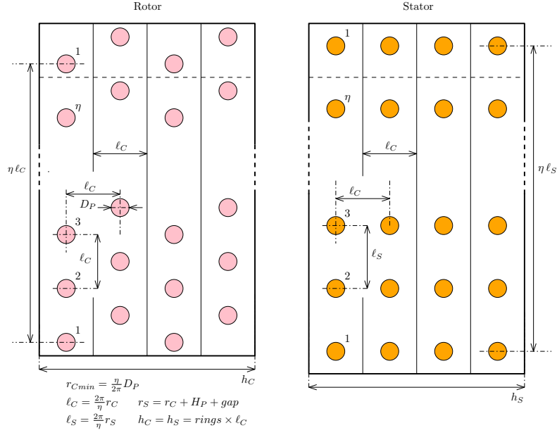
Fig. 4: Flat view of stator and staggered rotor rings.
