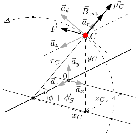
Fig. 8: Magnetic dipole momentum \vec{\mu}_C , which represents a disc-shaped permanent magnet (PM) as located in the rotor rings of Fig. 2, interacting with an external radial magnetic field, \vec{B}_{\text{ext}} , under mechanical angular vibrations \phi'_S .
