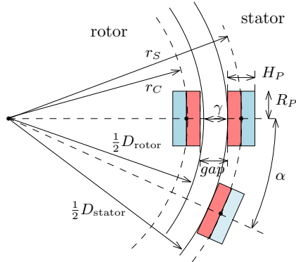
Fig. 3: Geometrical quantities of rotor and stator with face-to-face magnets. D_{\text{rotor}} is the outer diameter of the rotor, D_{\text{stator}} the inner diameter of the stator, and \text{gap} the separation between magnet faces. The disc PMs are recessed below the rotor and stator surfaces to obtain aerodynamic smoothing, therefore \gamma < \text{gap} .
