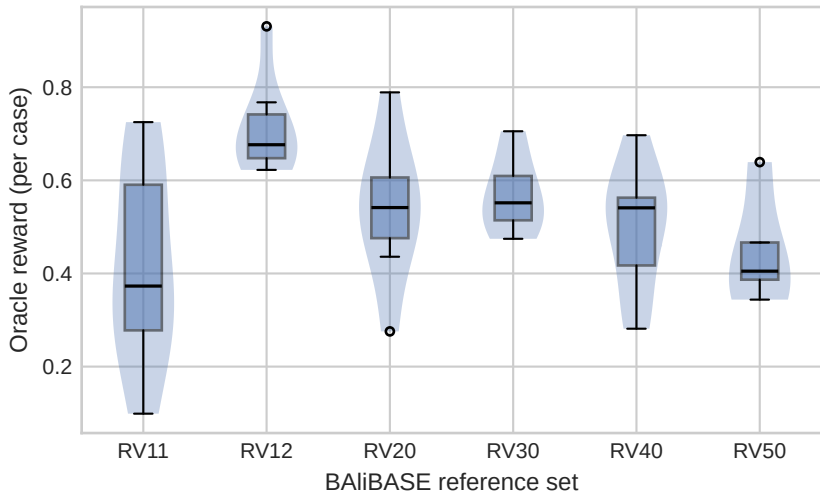
Fig S6: Reward Distribution by Dataset
