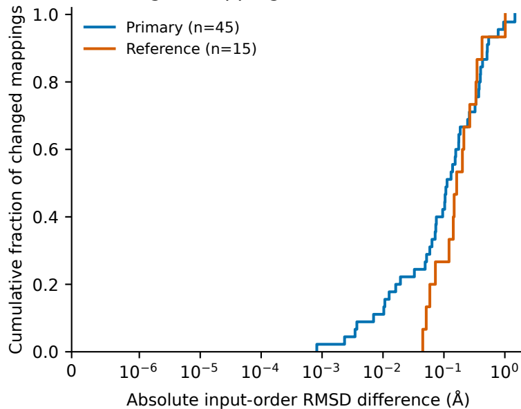
B Changed mappings: full
