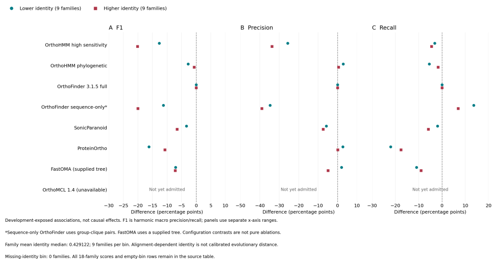
QfO SwissTrees: Sequence identity Descriptive differences versus full OrthoFinder 3.1.5; no subgroup confidence intervals or significance tests.
