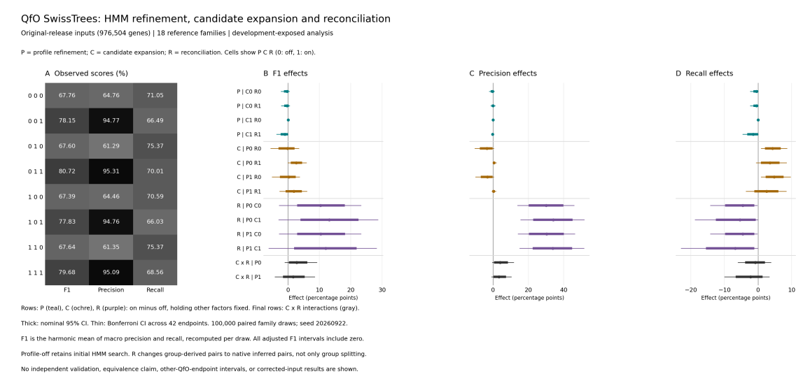
Figure: original-release SwissTrees cell scores and all 42 prespecified conditional-effect and interaction endpoints. Thick intervals are nominal 95% paired family intervals; thin intervals retain Bonferroni adjustment. Effects are shown in percentage points, including C-by-R differences of differences. This is not the corrected-input rerun or a comparison against OrthoFinder. The figure manifest binds the generated PNG/PDF/SVG files to their exact source result and plotter.
