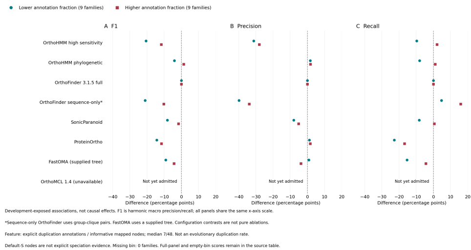
QfO SwissTrees: mapped-tree duplication annotations Descriptive differences versus full OrthoFinder 3.1.5; no subgroup intervals or significance tests.
