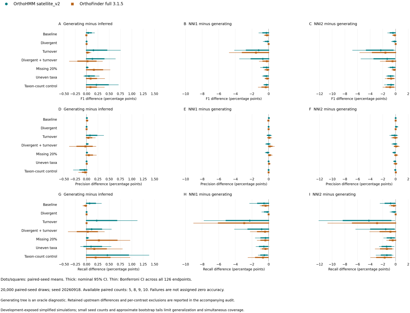
Figure: all126 exploratory F1, precision and recall endpoints across seven conditions, two methods and three tree contrasts. Points are paired-seed mean differences; thick intervals are nominal95% and thin intervals use Bonferroni adjustment over126 endpoints. Axes share scales down each contrast column. No best-tree selection or failed-score imputation was performed. The figure is generated from the complete verified summary with source/output hashes; PDF and SVG versions accompany the PNG.
