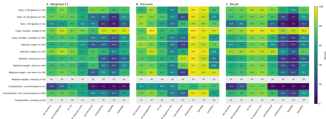
OrthoBench: all-method descriptive strata Eight retained methods | 14 frozen bins | 70 reference families | fixed method order
