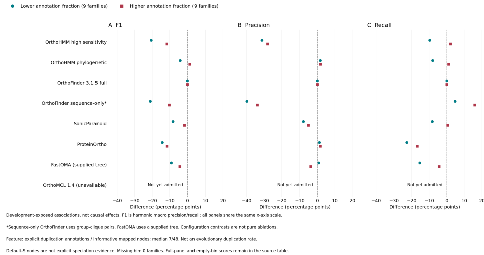
QfO SwissTrees: mapped-tree duplication annotations
