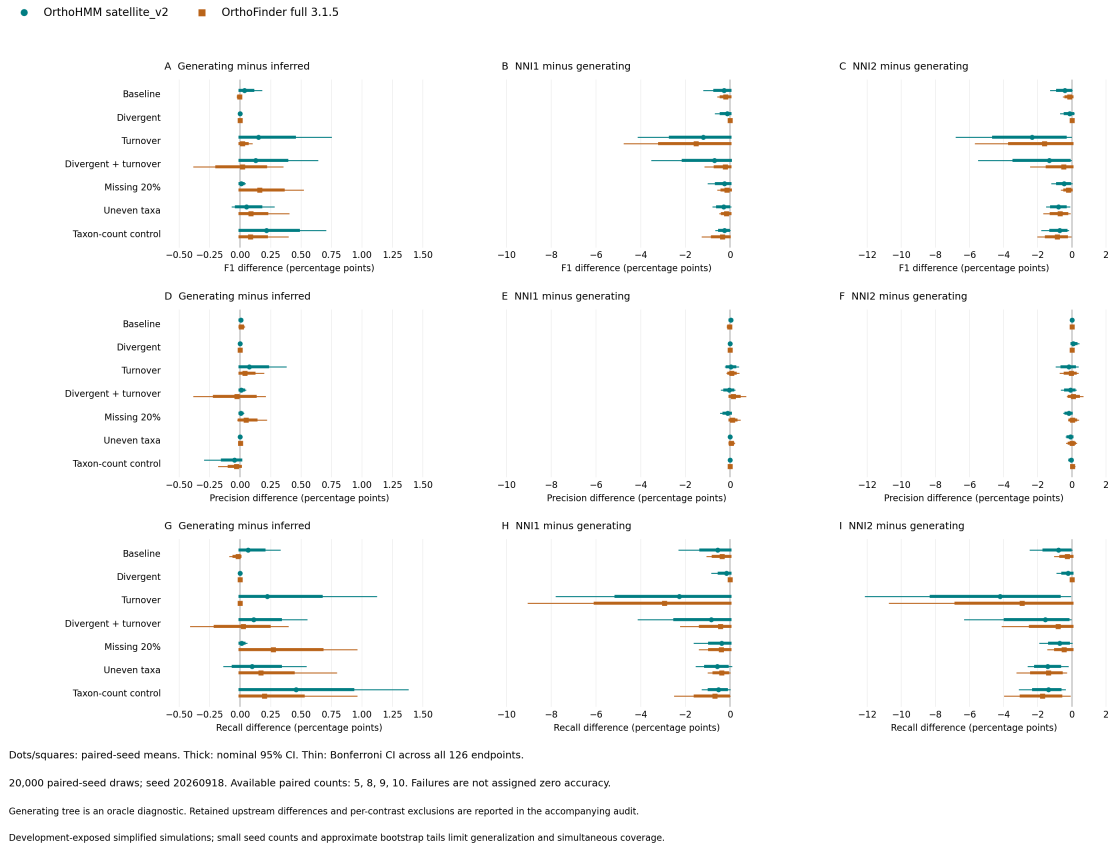
Figure: all 126 exploratory F1, precision and recall endpoints across seven conditions, two methods and three tree contrasts. Points are paired-seed mean differences; thick intervals are nominal 95% and thin intervals use Bonferroni adjustment over 126 endpoints. Axes share scales down each contrast column. No best-tree selection or failed-score imputation was performed. The figure is generated from the complete verified summary with source/output hashes; PDF and SVG versions accompany the PNG.
