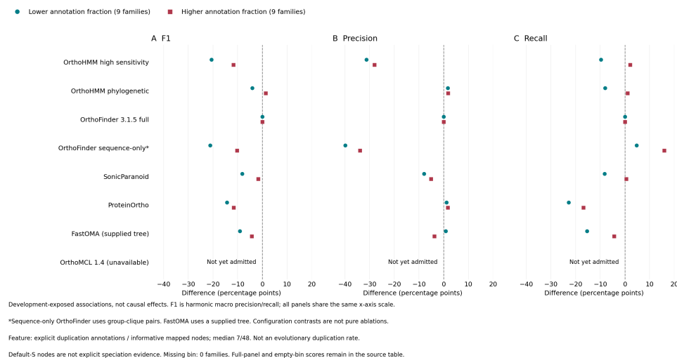
Ofo SwissTrees: mapped-tree duplication annotations
