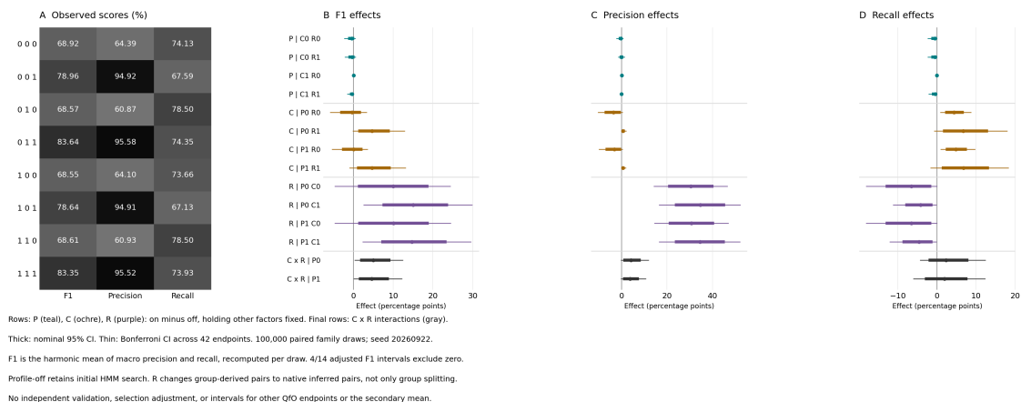
QfO SwissTrees: HMM refinement, candidate expansion and reconciliation Corrected-release inputs (984,137 genes) | 18 reference families | development-exposed analysis
