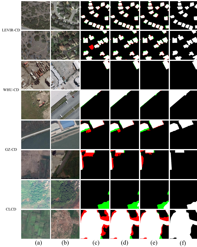
Fig. 10. Visualization comparisons of the effectiveness of PFEM and EARM. (a) T1 image. (b) T2 image. (c) Method-1. (d) Method-2. (e) SFEARNet. (f) Ground truth. White indicates true positive. Black indicates true negative. Red indicates false positive. Green indicates false negative.
