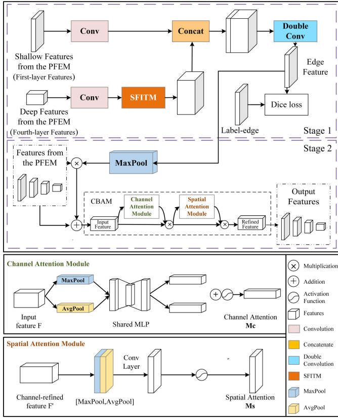
Fig. 4. Framework of EARM.
