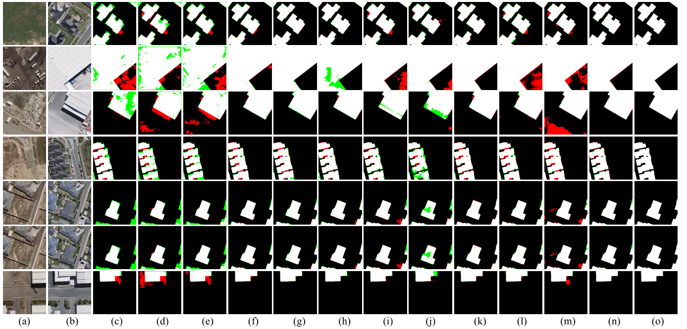
Fig. 6. Visualization comparisons on the WHU-CD dataset. (a) T1 image. (b) T2 image. (c) FC-EF. (d) FC-Siam-Conc. (e) FC-Siam-Diff. (f) STANet. (g) BIT. (h) MSCANet. (i) DESSN. (j) ChangeFormer. (k) AMTNet. (l) USSFC. (m) EATDer. (n) SFEARNet. (o) Ground truth. White indicates true positive. Black indicates true negative. Red indicates false positive. Green indicates false negative.
