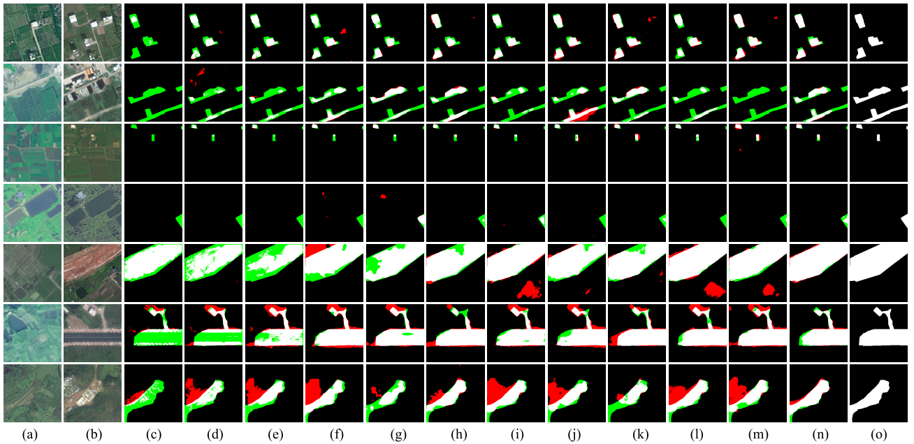
Fig. 8. Visualization comparisons on the CLCD dataset. (a) T1 image. (b) T2 image. (c) FC-EF. (d) FC-Siam-Conc. (e) FC-Siam-Diff. (f) STANet. (g) BIT. (h) MSCANet. (i) DESSN. (j) ChangeFormer. (k) AMTNet. (l) USSFC. (m) EATDer. (n) SFEARNet. (o) Ground truth. White indicates true positive. Black indicates true negative. Red indicates false positive. Green indicates false negative.
