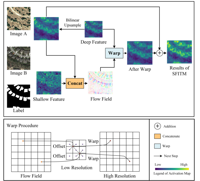
Fig. 2. Framework of SFITM.
