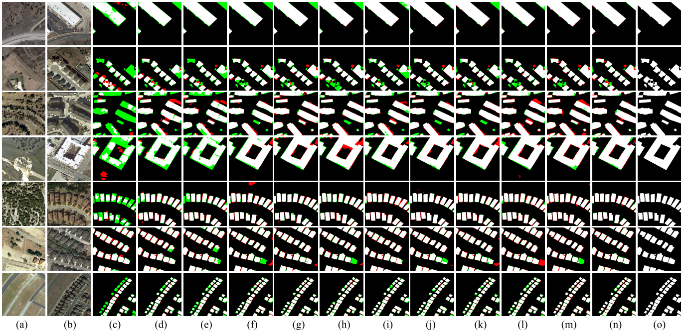
Fig. 5. Visualization comparisons on the LEVIR-CD dataset. (a) T1 image. (b) T2 image. (c) FC-EF. (d) FC-Siam-Conc. (e) FC-Siam-Diff. (f) STANet. (g) BIT. (h) MSCANet. (i) DESSN. (j) ChangeFormer. (k) AMTNet. (l) USSFC. (m) EATDer. (n) SFEARNet. (o) Ground truth. White indicates true positive. Black indicates true negative. Red indicates false positive. Green indicates false negative.
