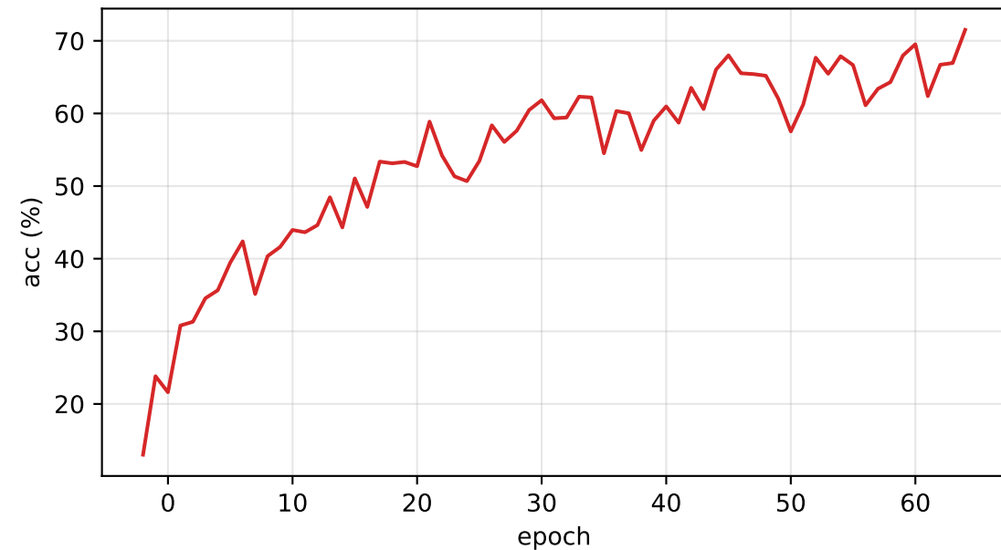
Backdoor Acc
