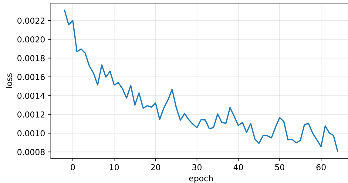
Backdoor Loss
