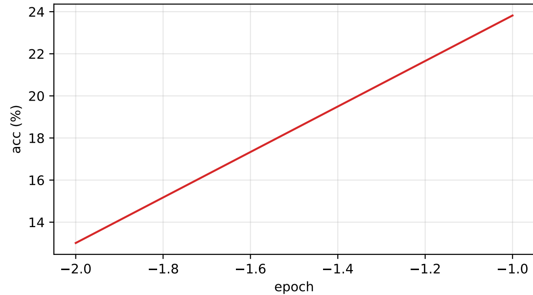
Backdoor Acc
