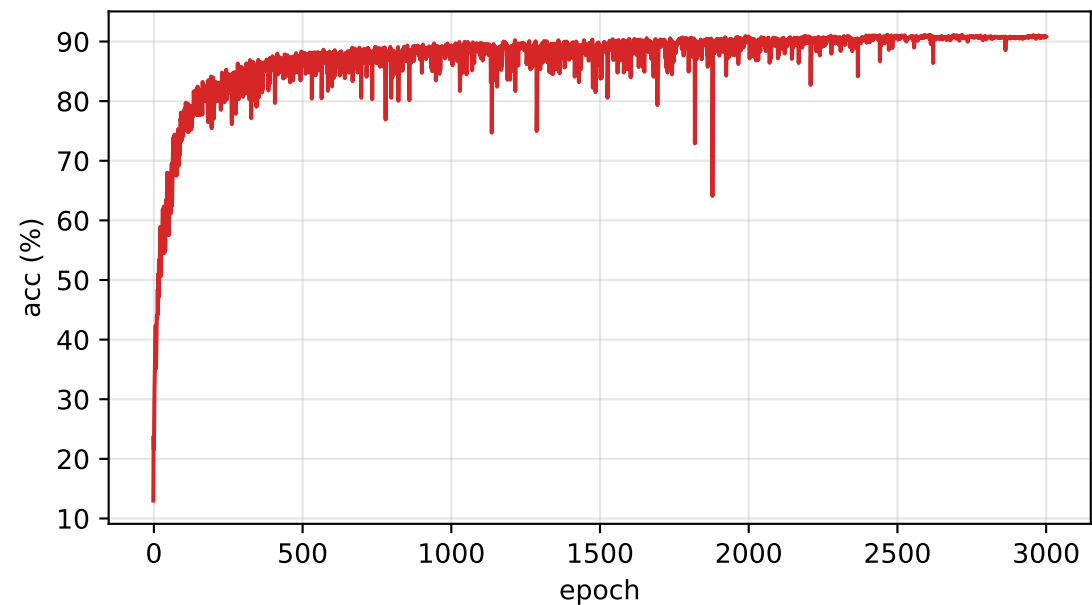
Backdoor Acc
