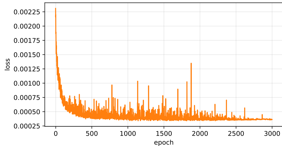
Backdoor Loss
