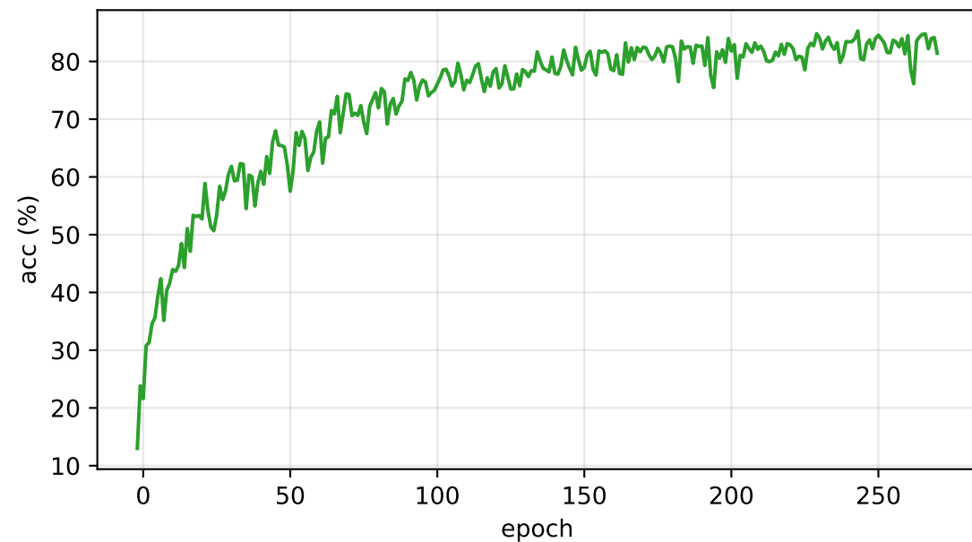
Backdoor Acc
