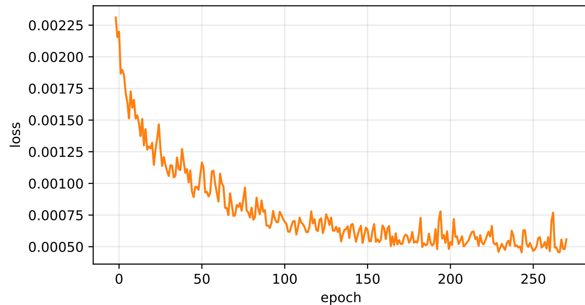
Backdoor Loss
