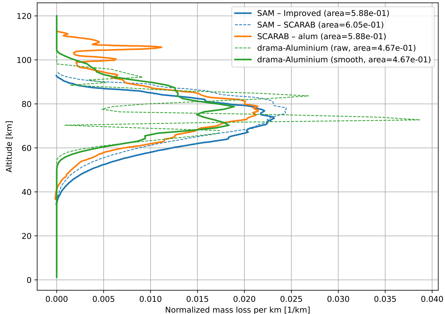
Model comparison for normalized aluminium deposition
