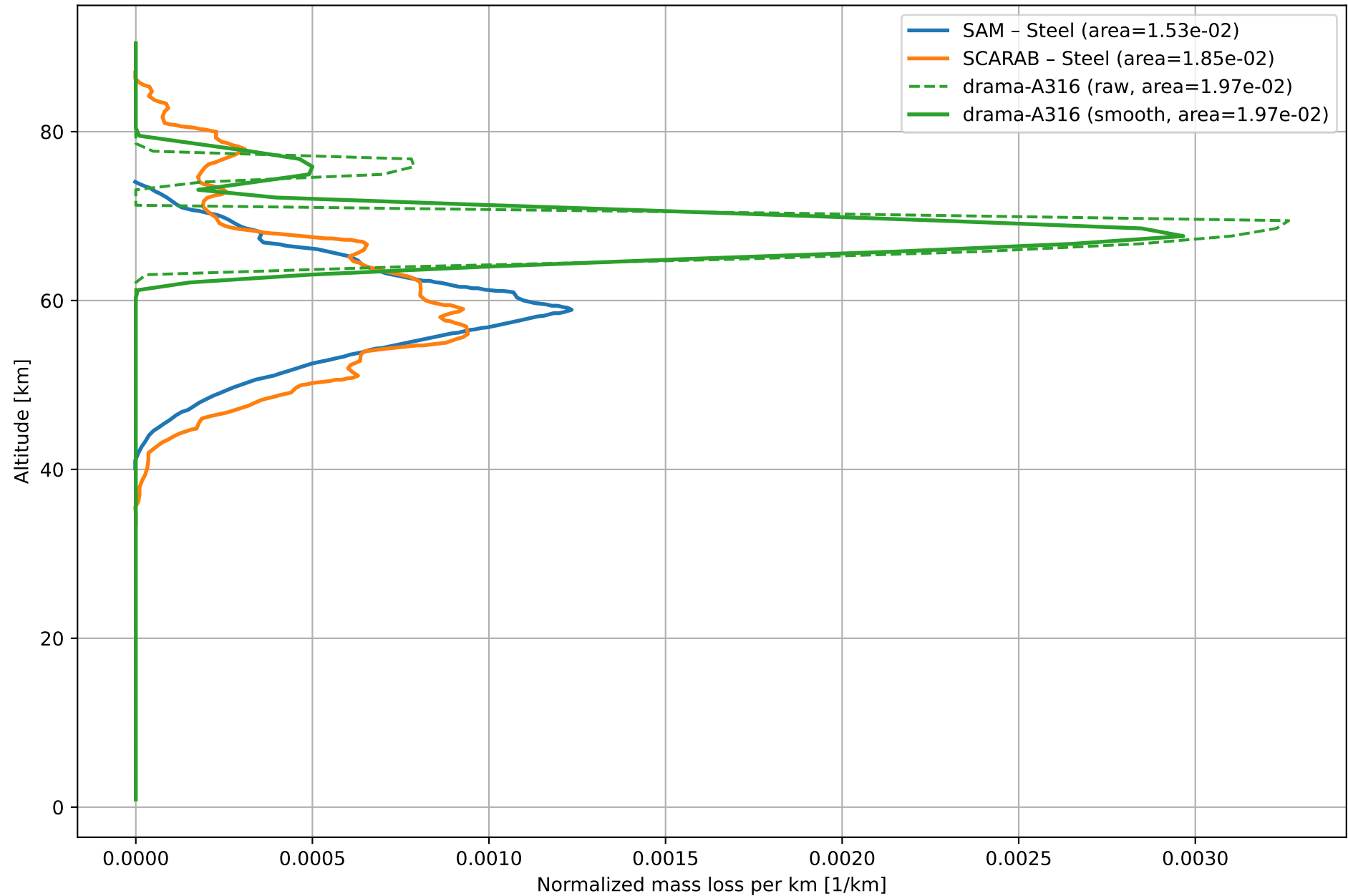
Steel model comparison
