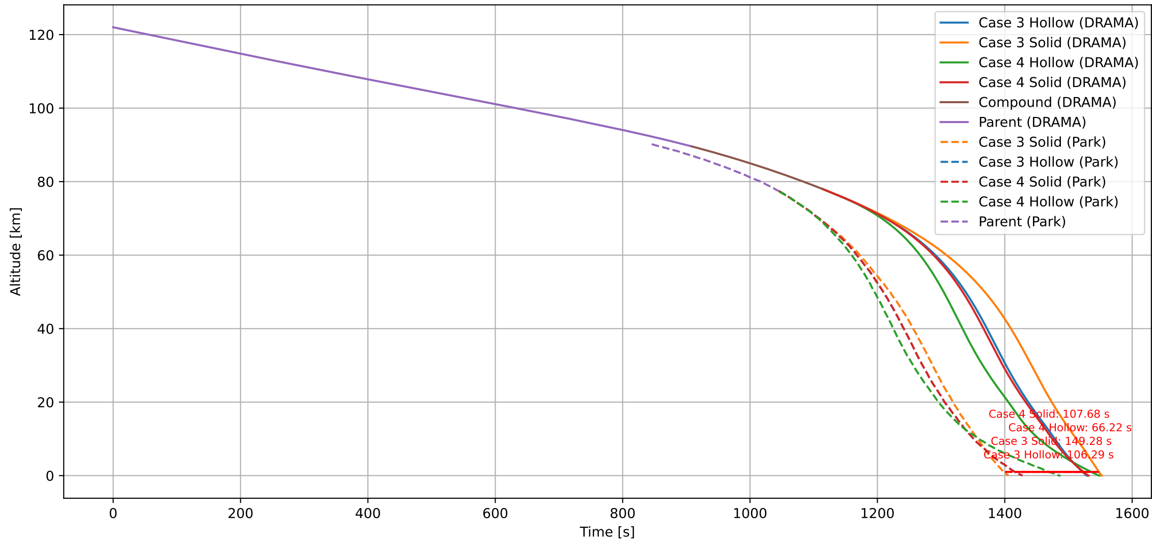
Comparison: DRAMA vs Park(EQ) — Altitude vs Time (With Differences)
