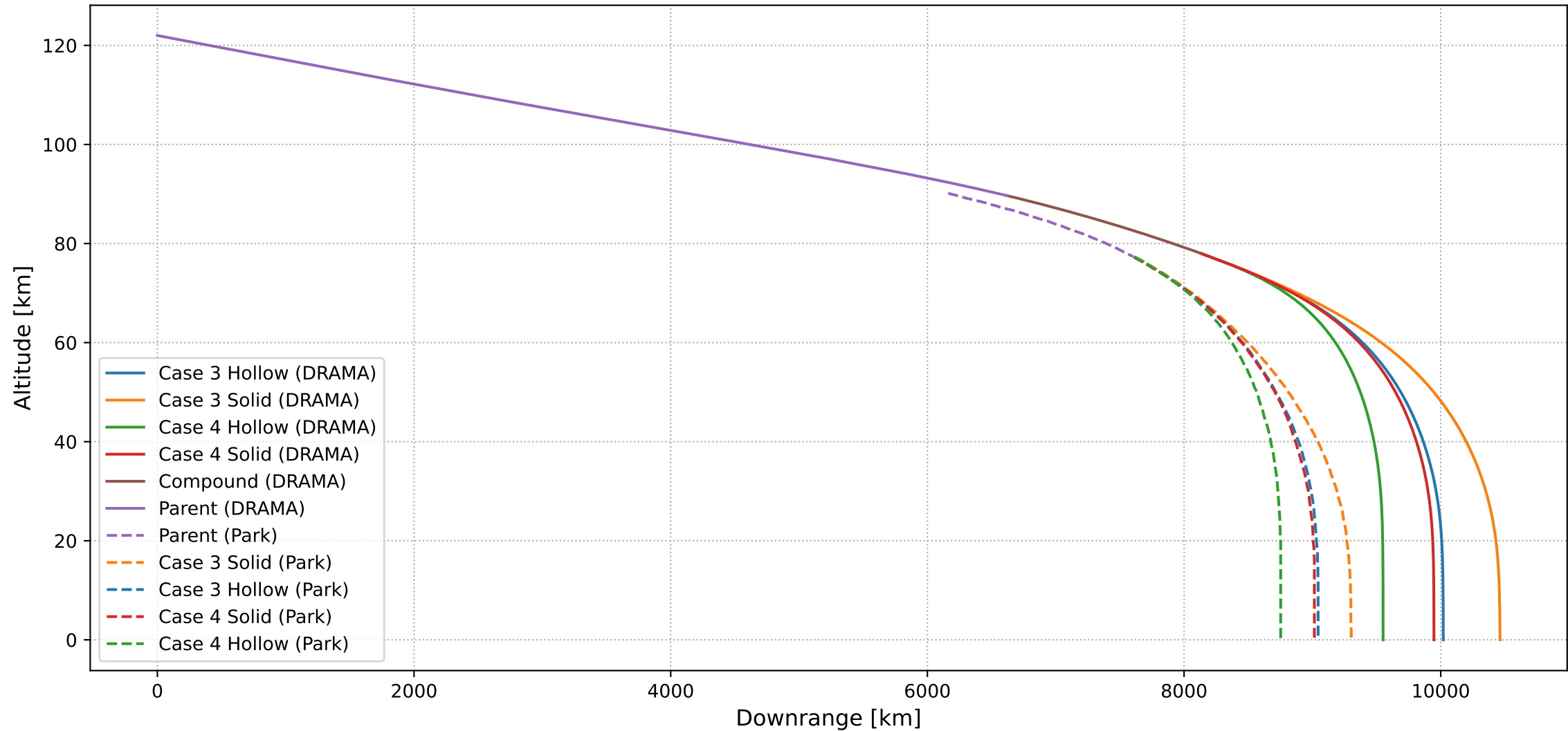
Comparison: DRAMA vs Park (EQ) — Altitude vs Downrange
