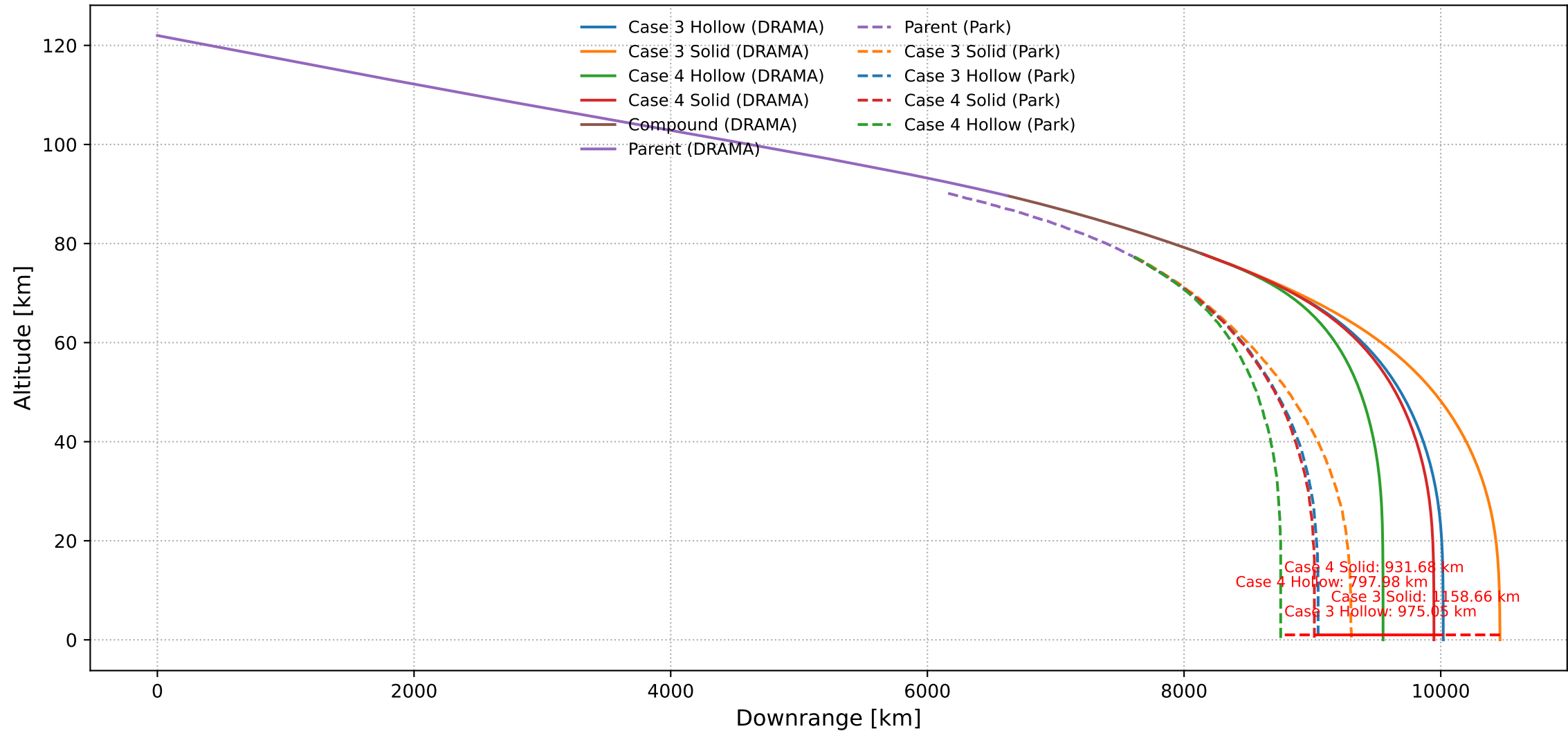
Comparison: DRAMA vs PARK (EQ) — Altitude vs Downrange (With Differences)
