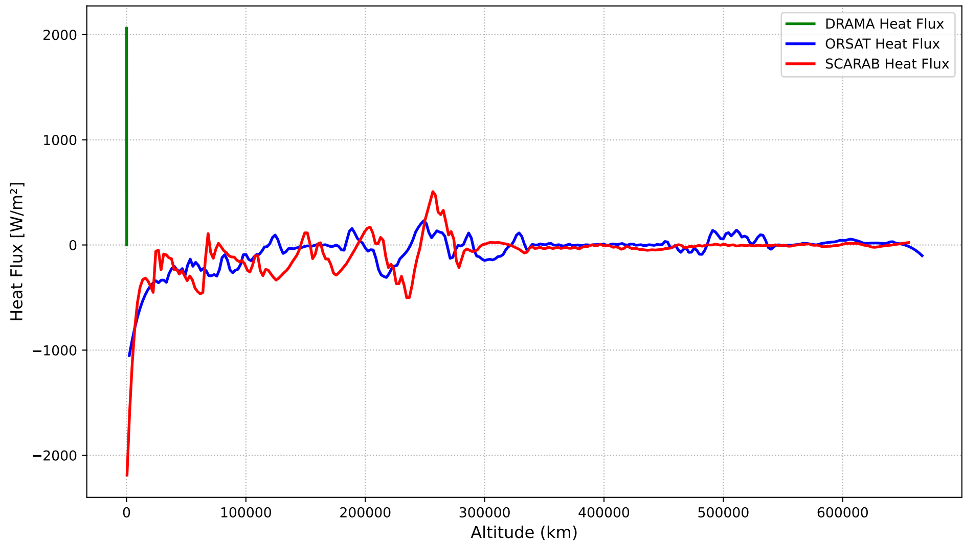
Smooth Heat Flux vs Altitude
