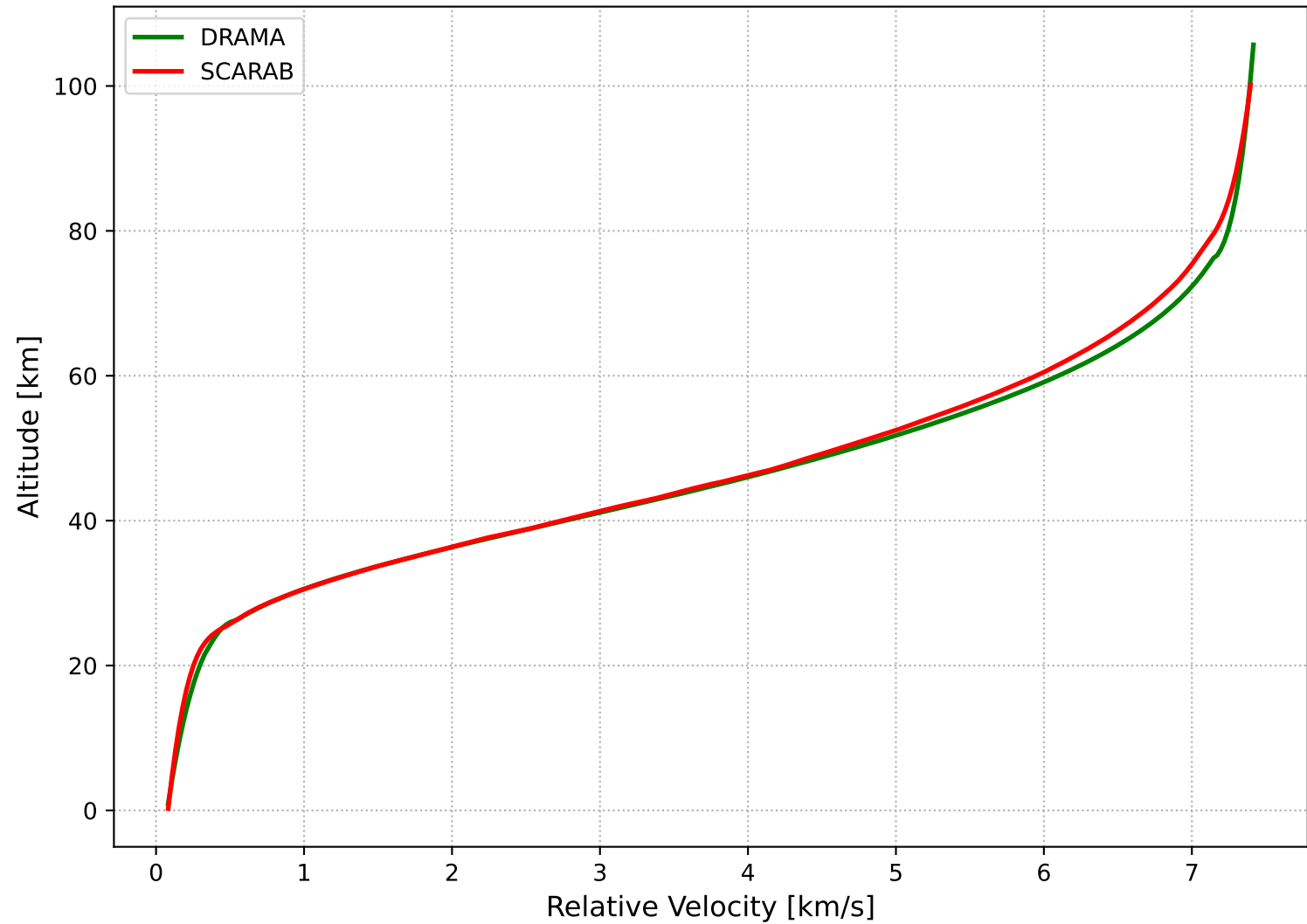
Velocity vs Altitude
