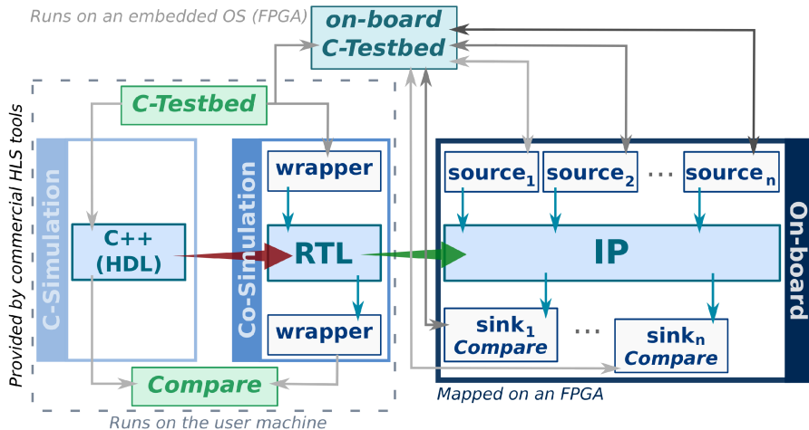
Figure: FPGA-Based Solution for On-Board Verification of Hardware Modules Using HLS
