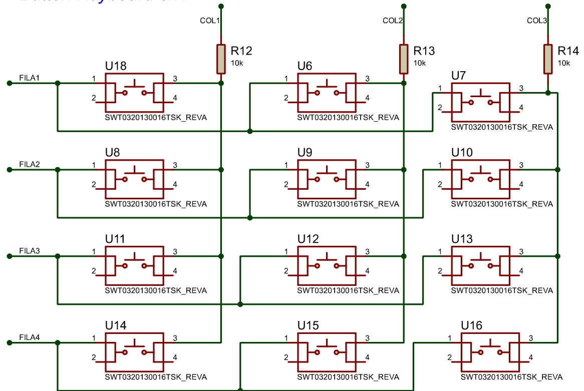
Button Keyboard 3x4
