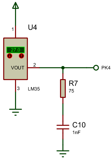
LM35 Temperature Sensor
