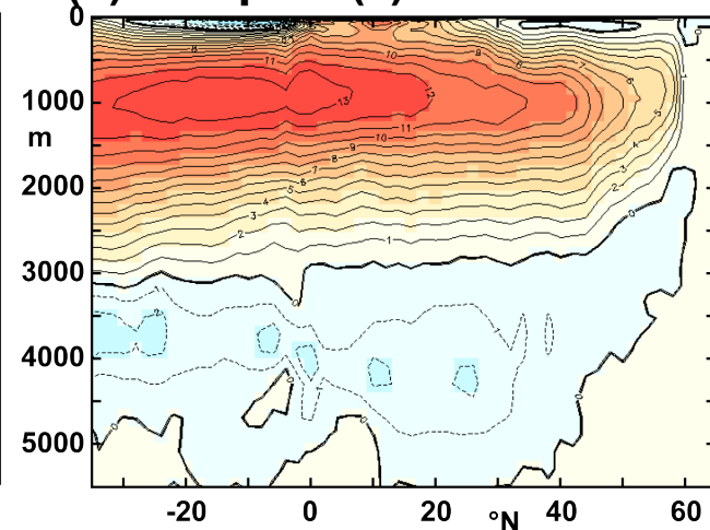
(c) GS1p2 \Psi(z)
