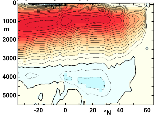
(b) GS1p1 \Psi(z)
