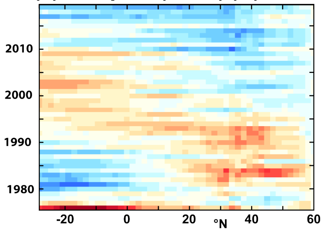
(e) GS1p1 \Psi(z) - \langle \Psi(z) \rangle
