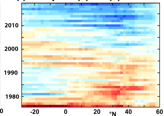
(f) GS1p2 \Psi(z) - \langle \Psi(z) \rangle
