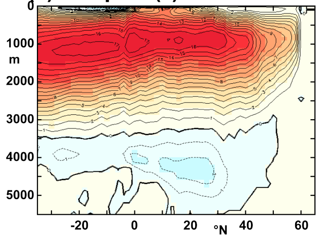
(a) GS1p0 \Psi(z)
