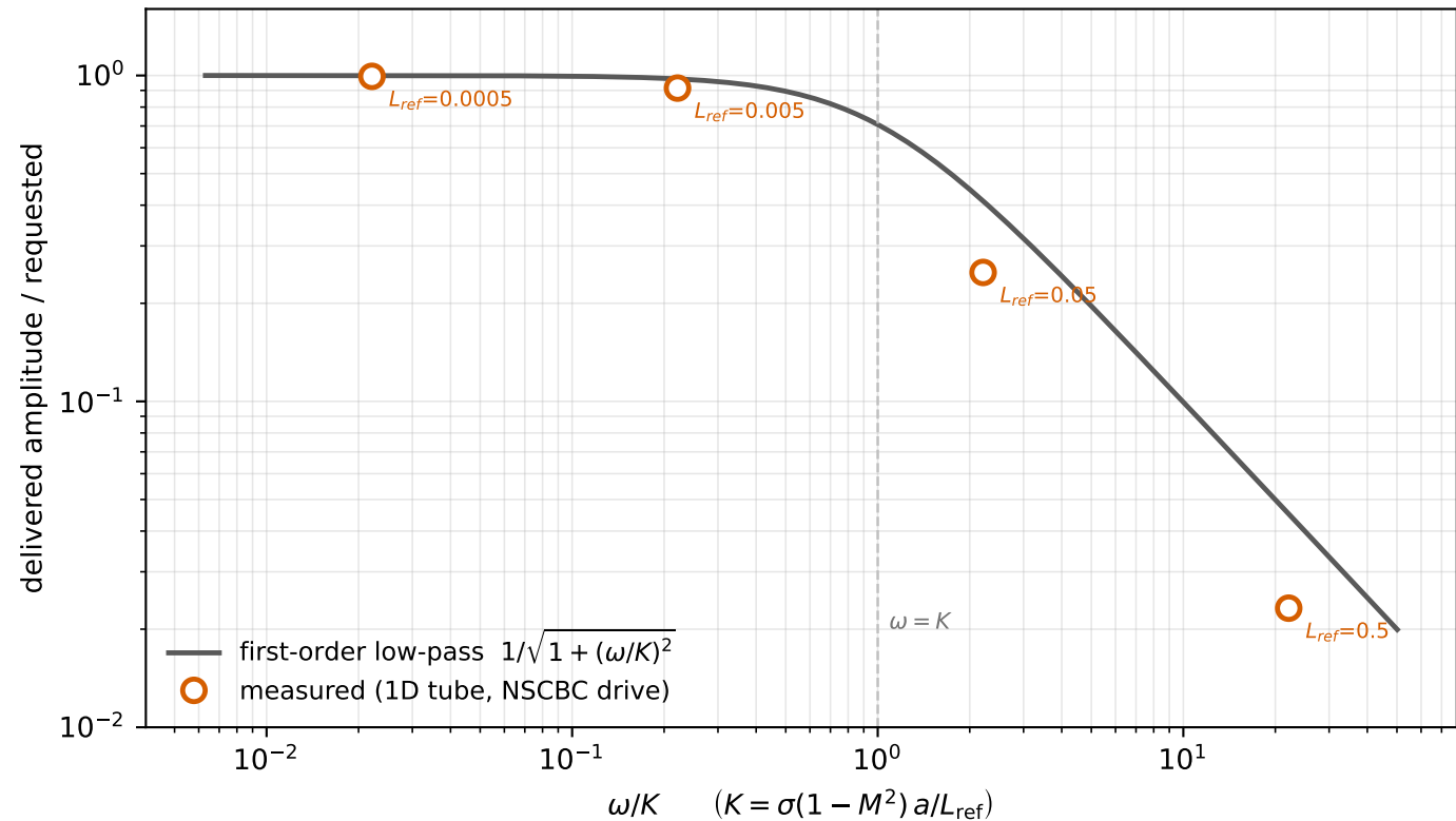
NSCBC drive is a first-order low-pass on the requested pressure
