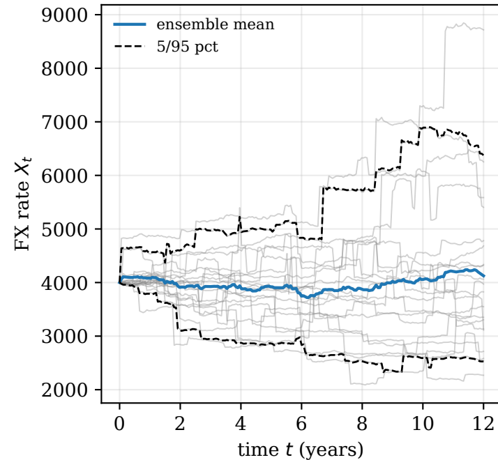
Merton: x_0 = 4000 , \sigma = 0.0144 , \lambda = 1.0 , T = 12
