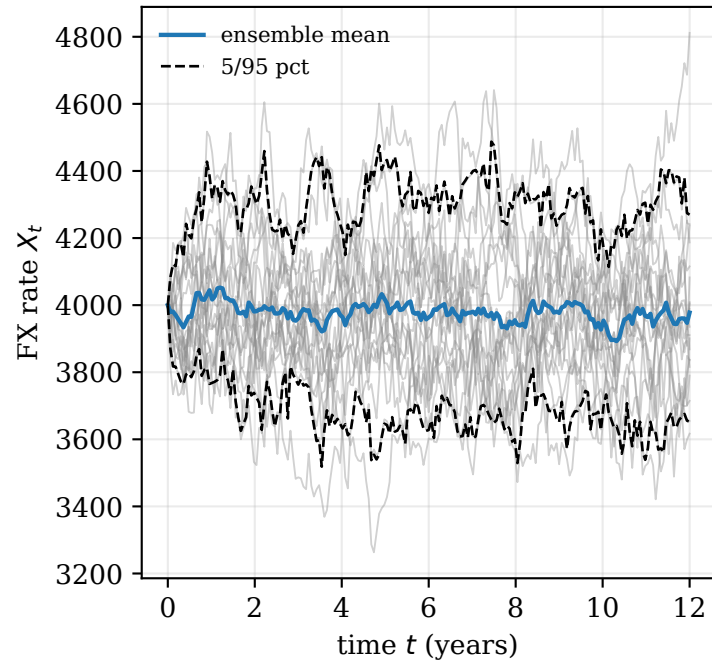
Ou: x_0 = 4000 , \bar{\mu} = 4000 , \theta = 1.0 , T = 12
