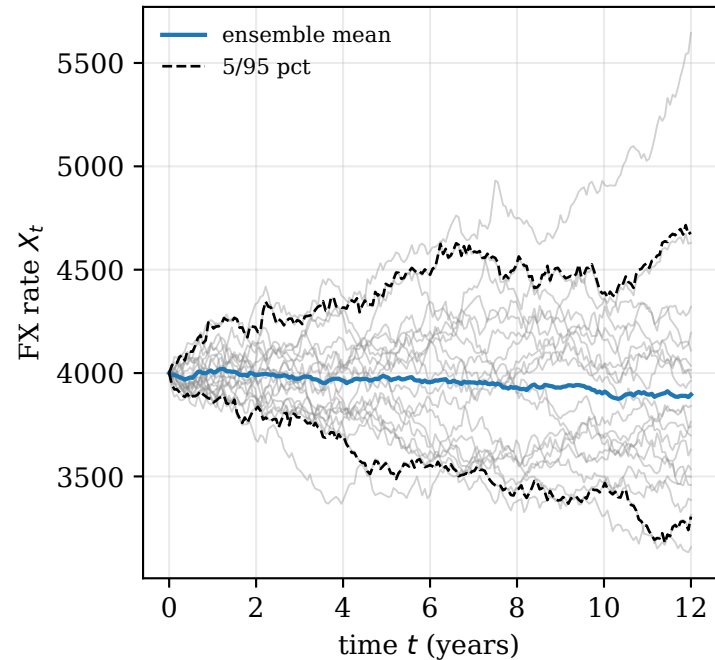
GBM: x_0 = 4000 , \sigma = 0.0289 , T = 12
