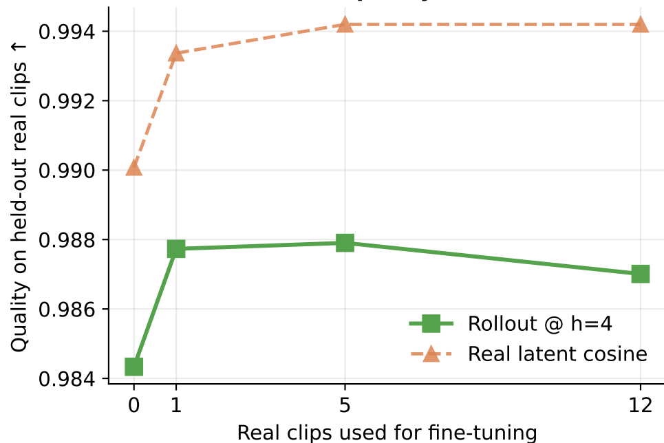
Rollout & latent quality vs data volume
