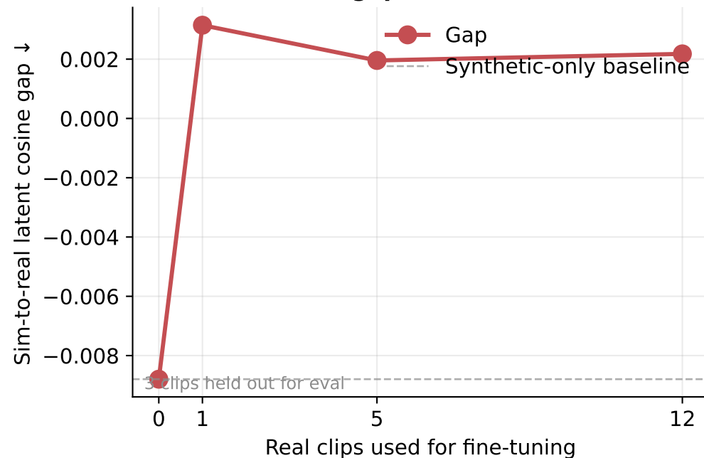
Transfer gap vs data volume
