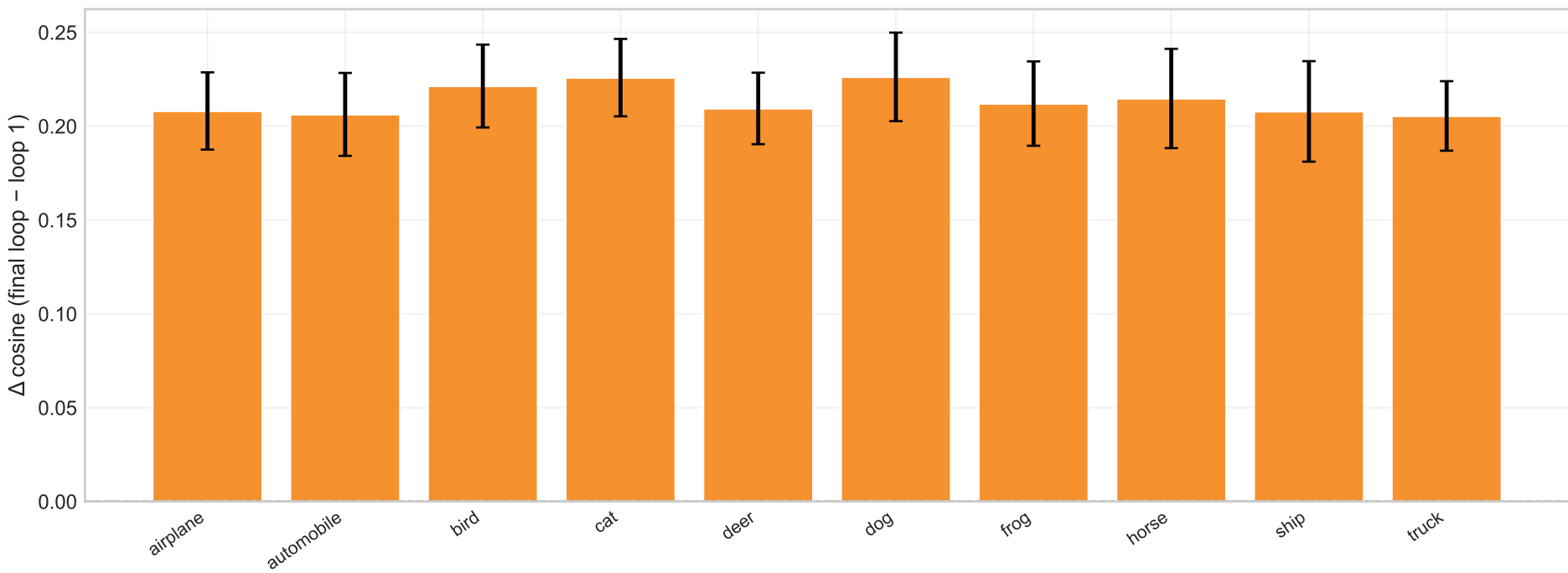
Per-class benefit from recurrence
