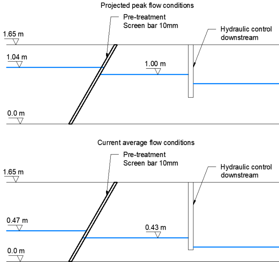
Figure 2: Preliminary treatment, screens section.
