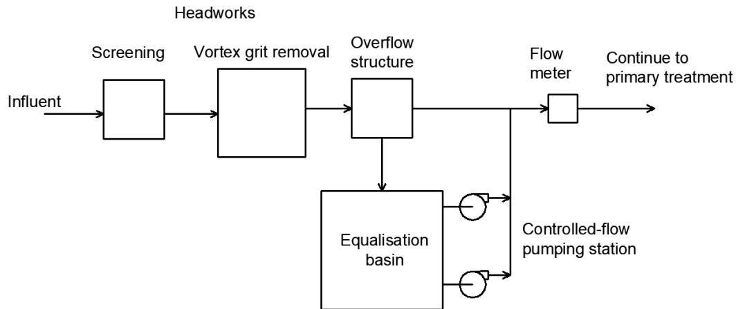
Figure 4: Off-line equalization basin –adapted from Fig 3-20, Davis,2010.
