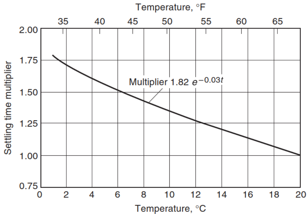
Figure 6: Temperature multiplier for retention time [?].
