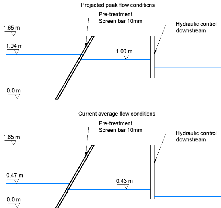
Figure 2: Preliminary treatment, screens section.
