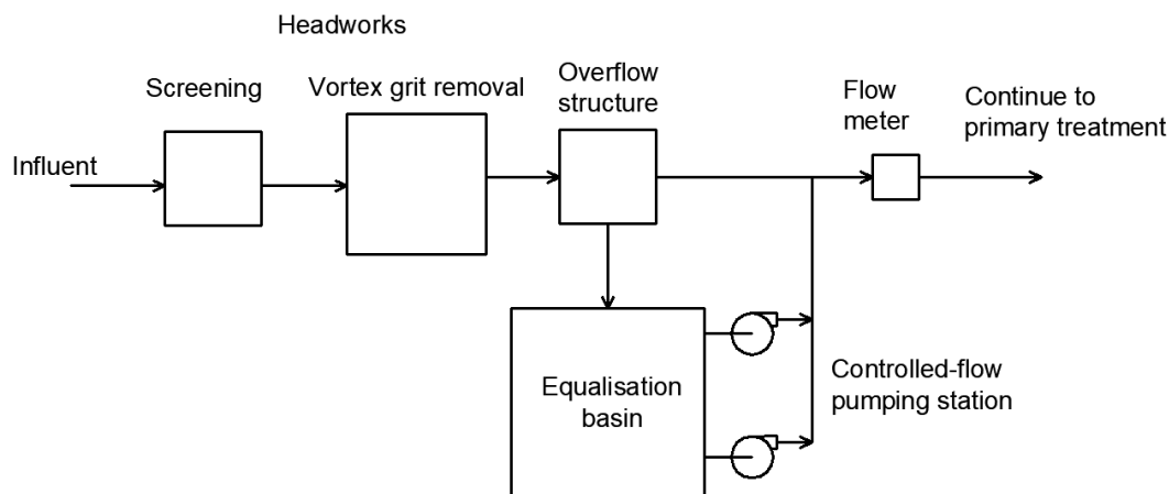
Figure 3: Off-line equalization basin –adapted from Fig 3-20, Davis, 2010.
