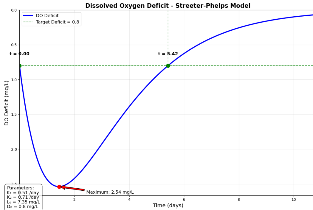
Figure 4: Dissolved oxygen deficit. Vertical axes being the deficit, with zero representation saturation.
