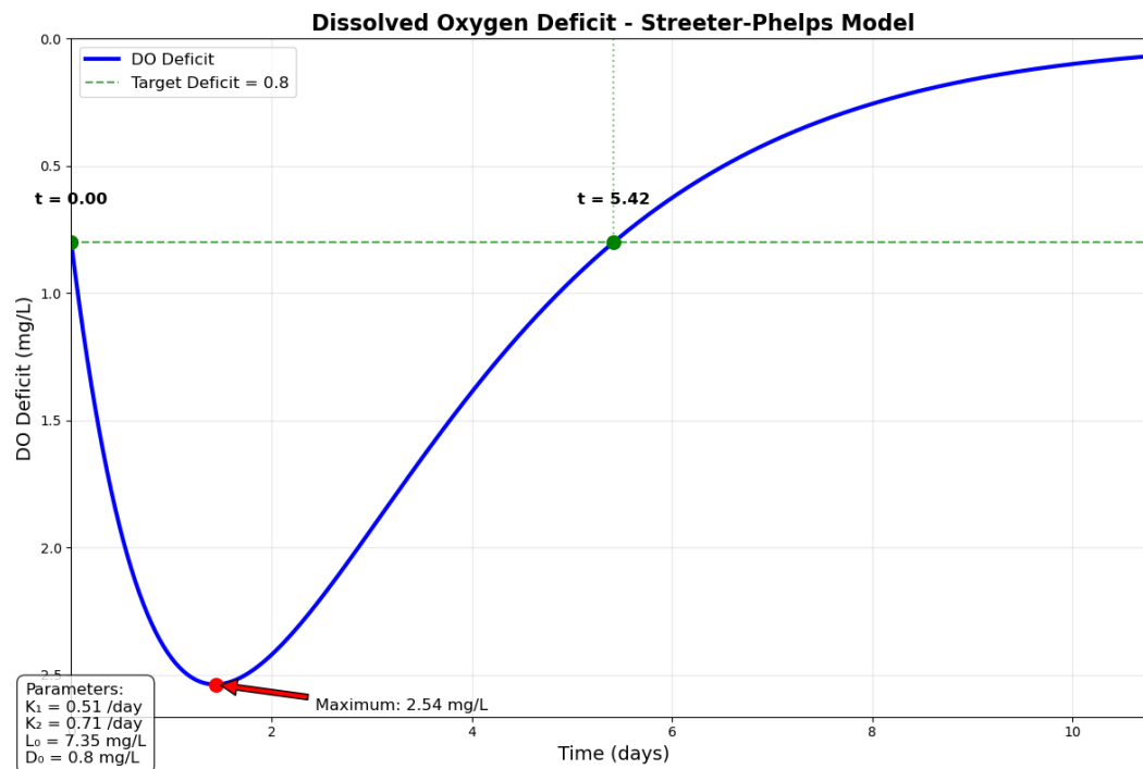
Figure 1: Dissolved oxygen deficit. Vertical axes being the deficit, with zero representation saturation.
