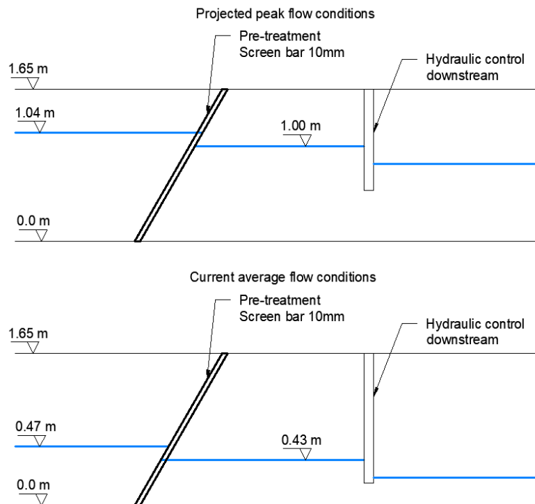
Figure 4: Preliminary treatment, screens section.
