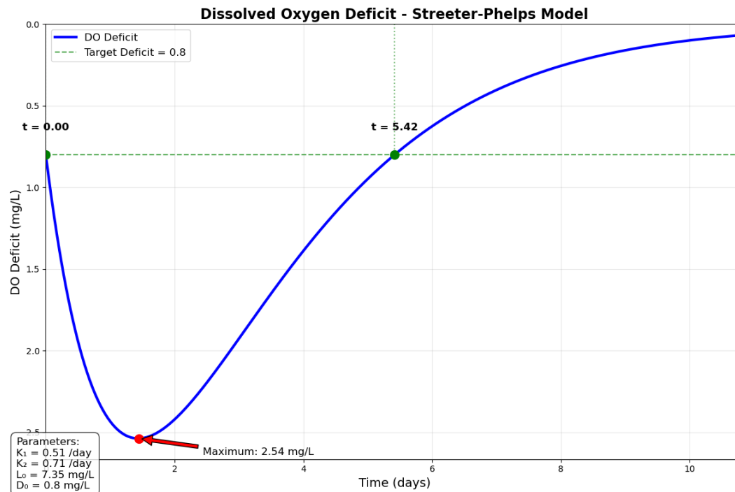
Figure 2: Dissolved oxygen deficit. Vertical axes being the deficit, with zero representation saturation.
