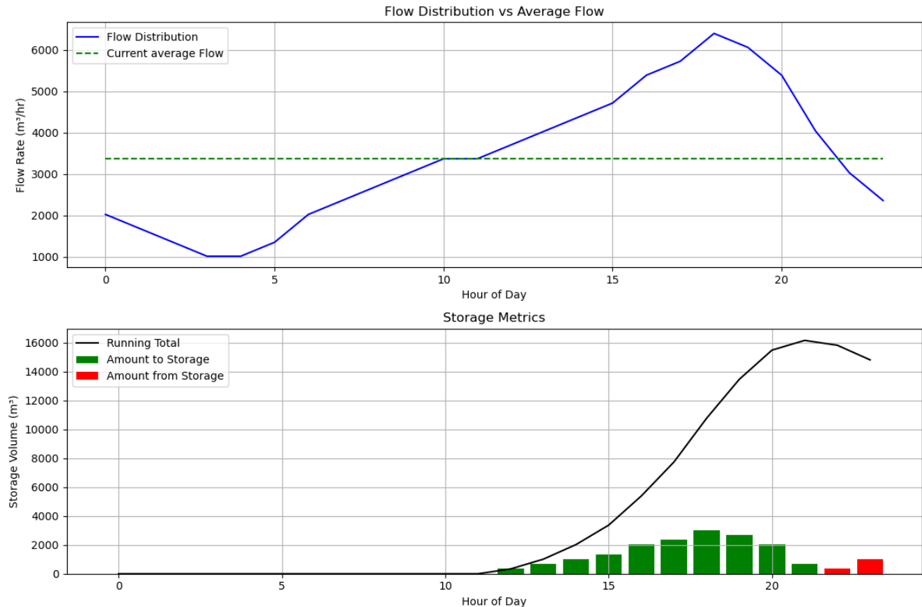
Figure 8: Mass balance diagram for current conditions.
