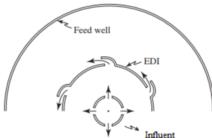
Figure 4: Feed well with energy dissipating inlet (EDI), plan view [Metcalf and Eddy, 2014].
