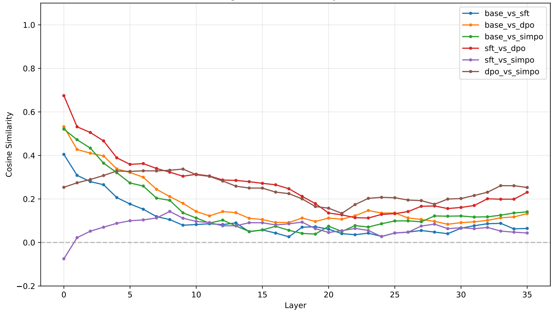
Probe Weight Direction Similarity Across Models
