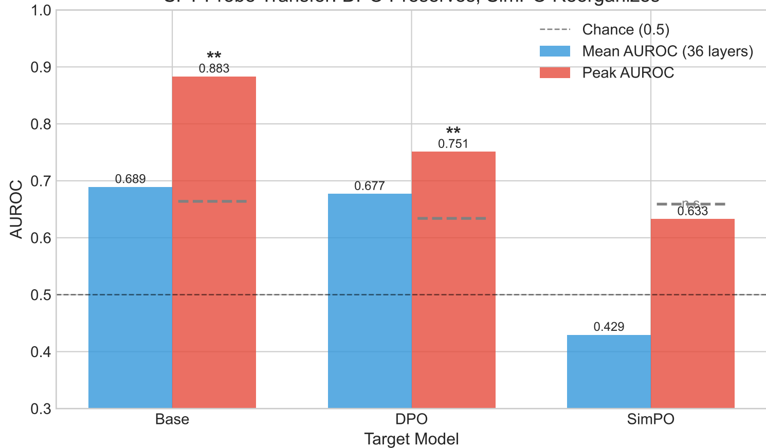
SFT Probe Transfer: DPO Preserves, SimPO Reorganizes
