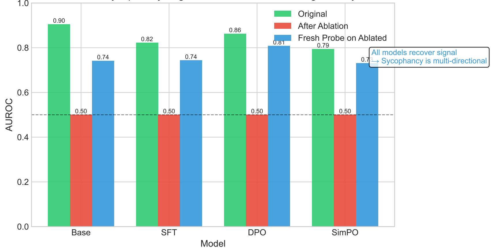
Multi-Directional Sycophancy: Signal Persists After Removing Primary Direction
