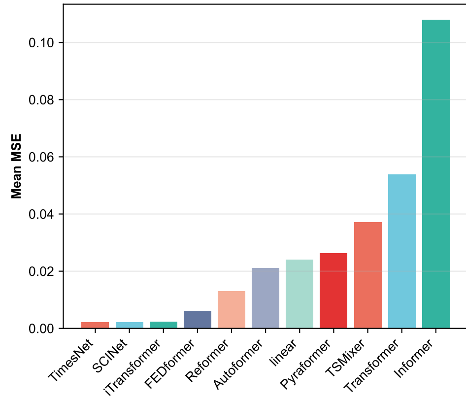
(C) Prediction Error by Model
