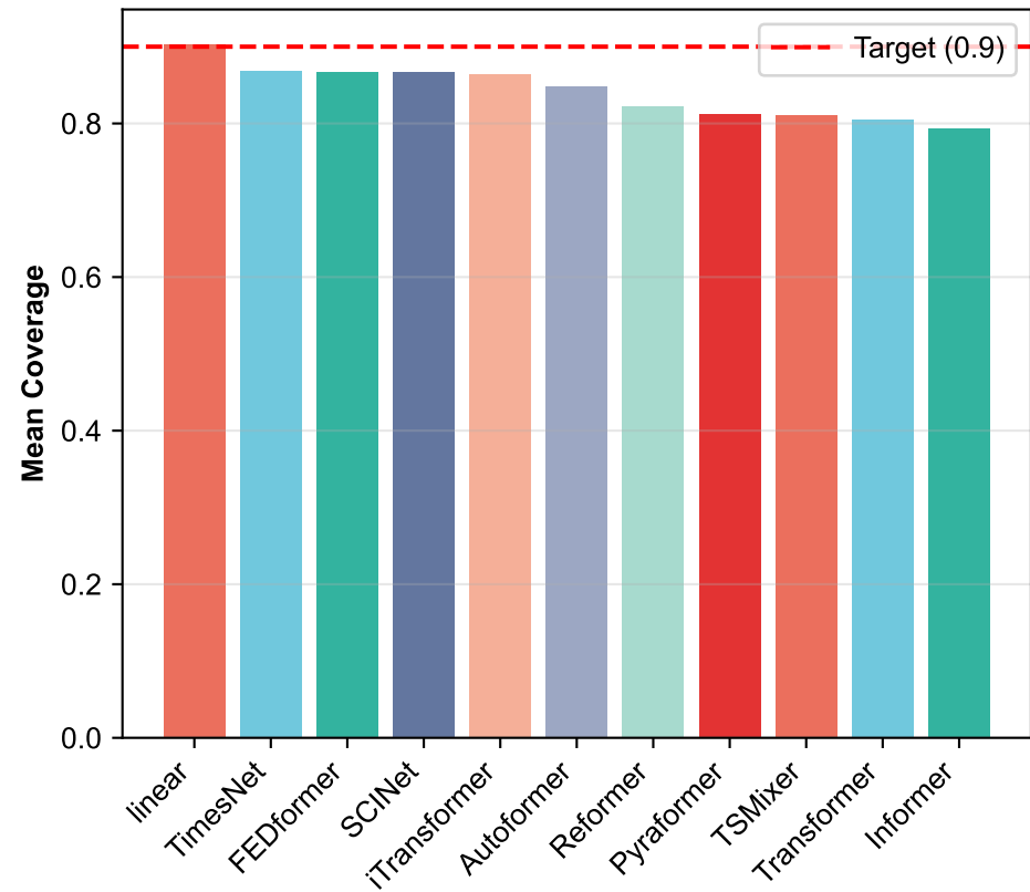
(A) Coverage by Model
