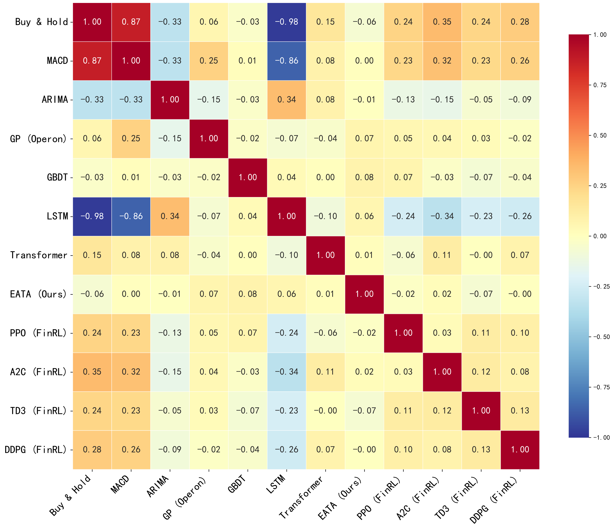
Strategy Correlation Matrix (All 12 Methods)
