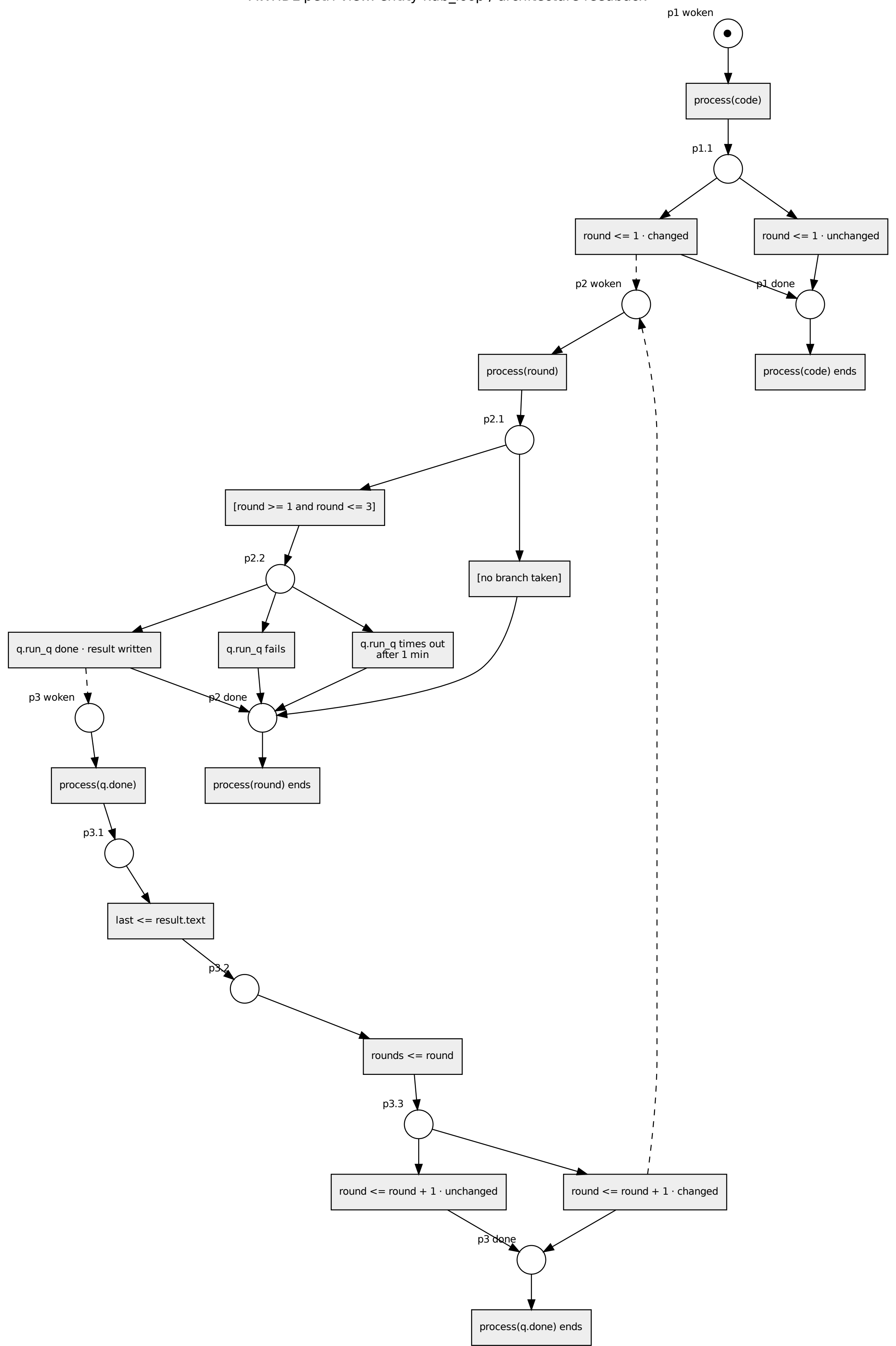
AWHDL petri view: entity kdb_loop / architecture feedback
