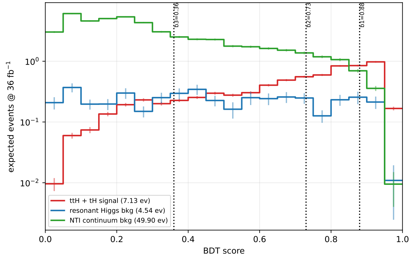
BDT score: expected model components with category boundaries
