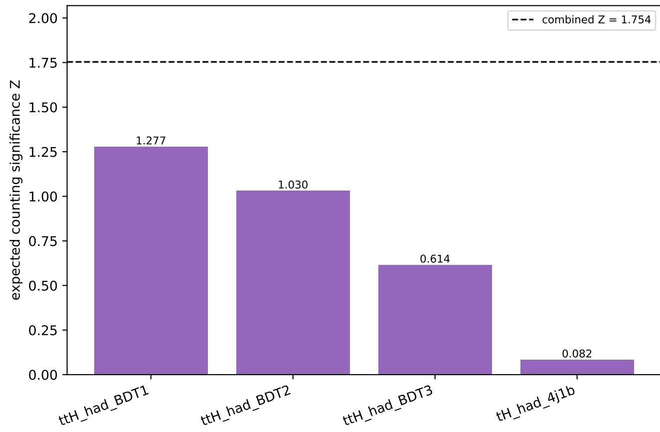
Expected counting significance per category @ 36 \text{ fb}^{-1}
