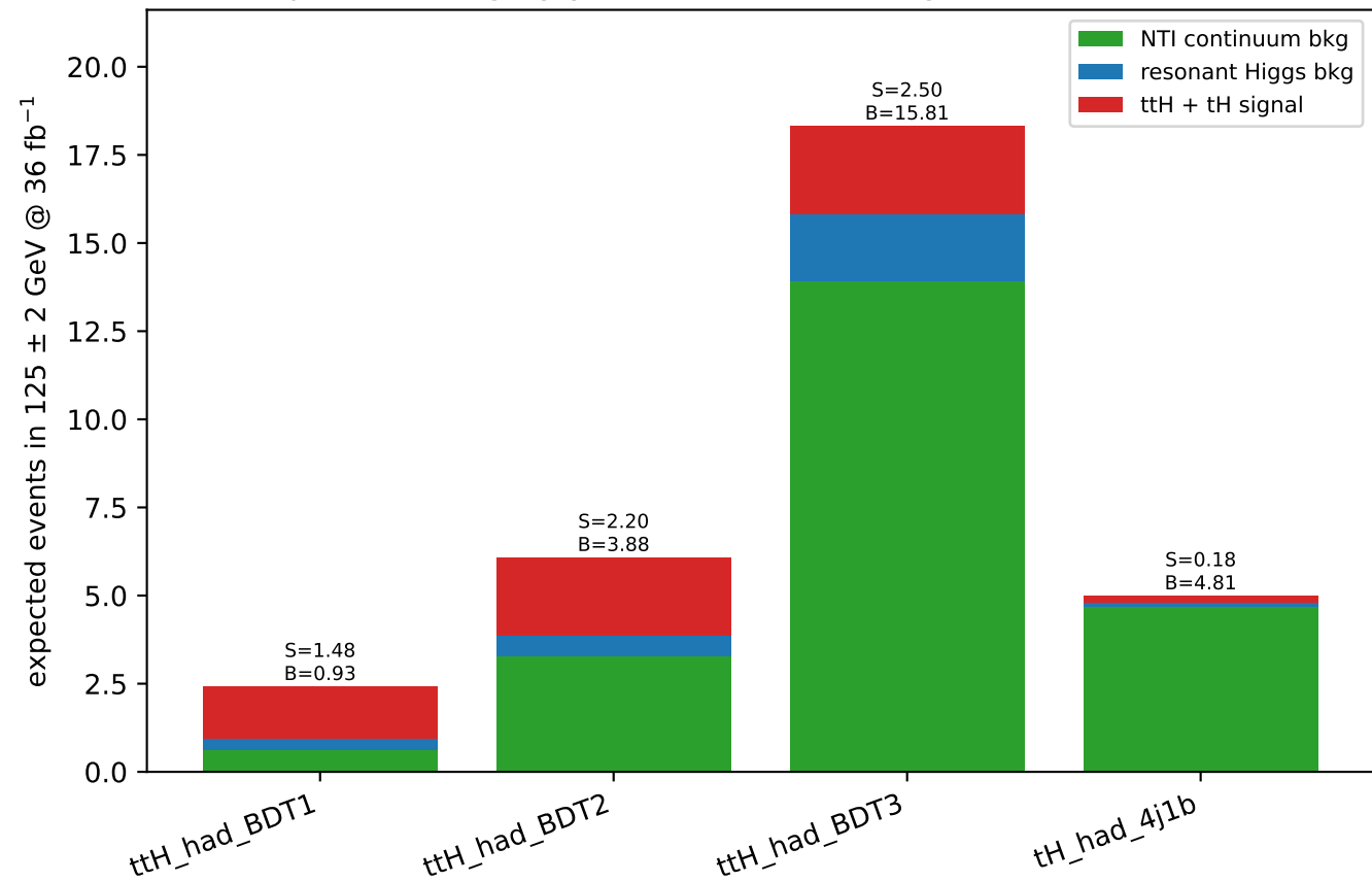
Expected category yields (observed TI signal window blinded)
