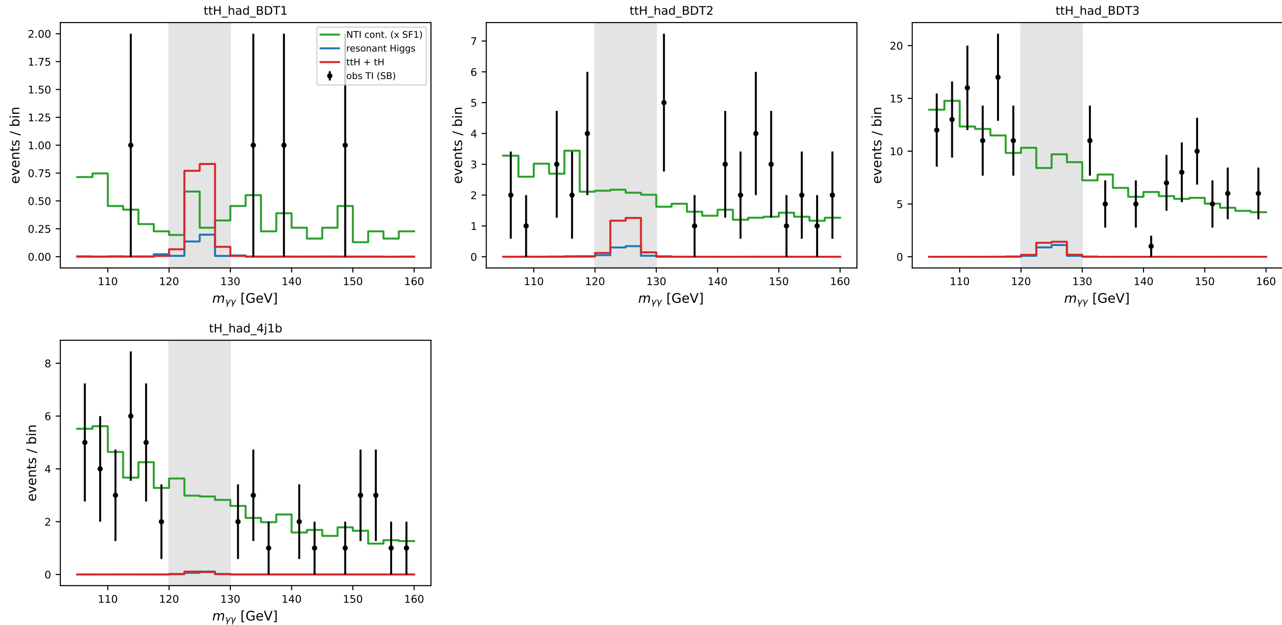
Per-category m_{\gamma\gamma} control shapes (grey band = blinded observed TI window; NTI unblinded)
